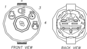
IGNITION SWITCH
