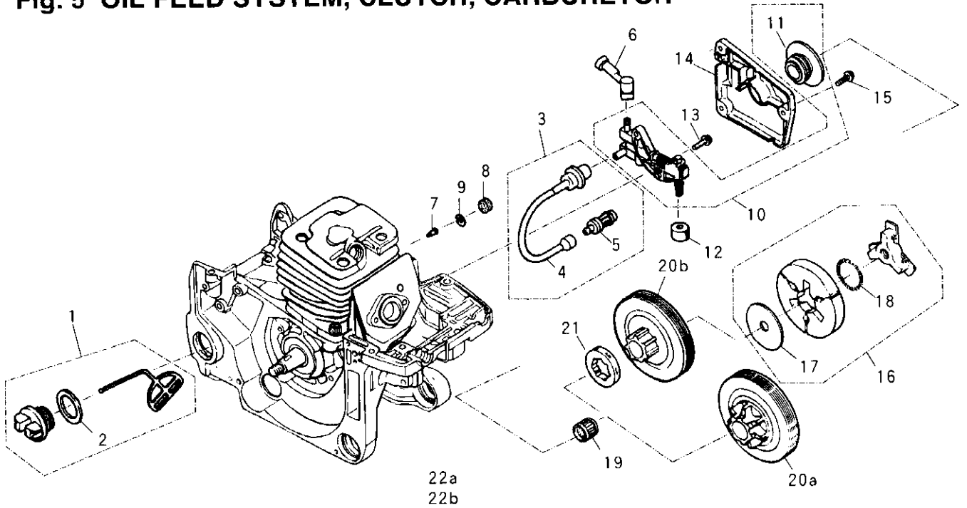
Fig. 5 OIL FEED SYSTEM, CLUTCH, CARBURETOR
