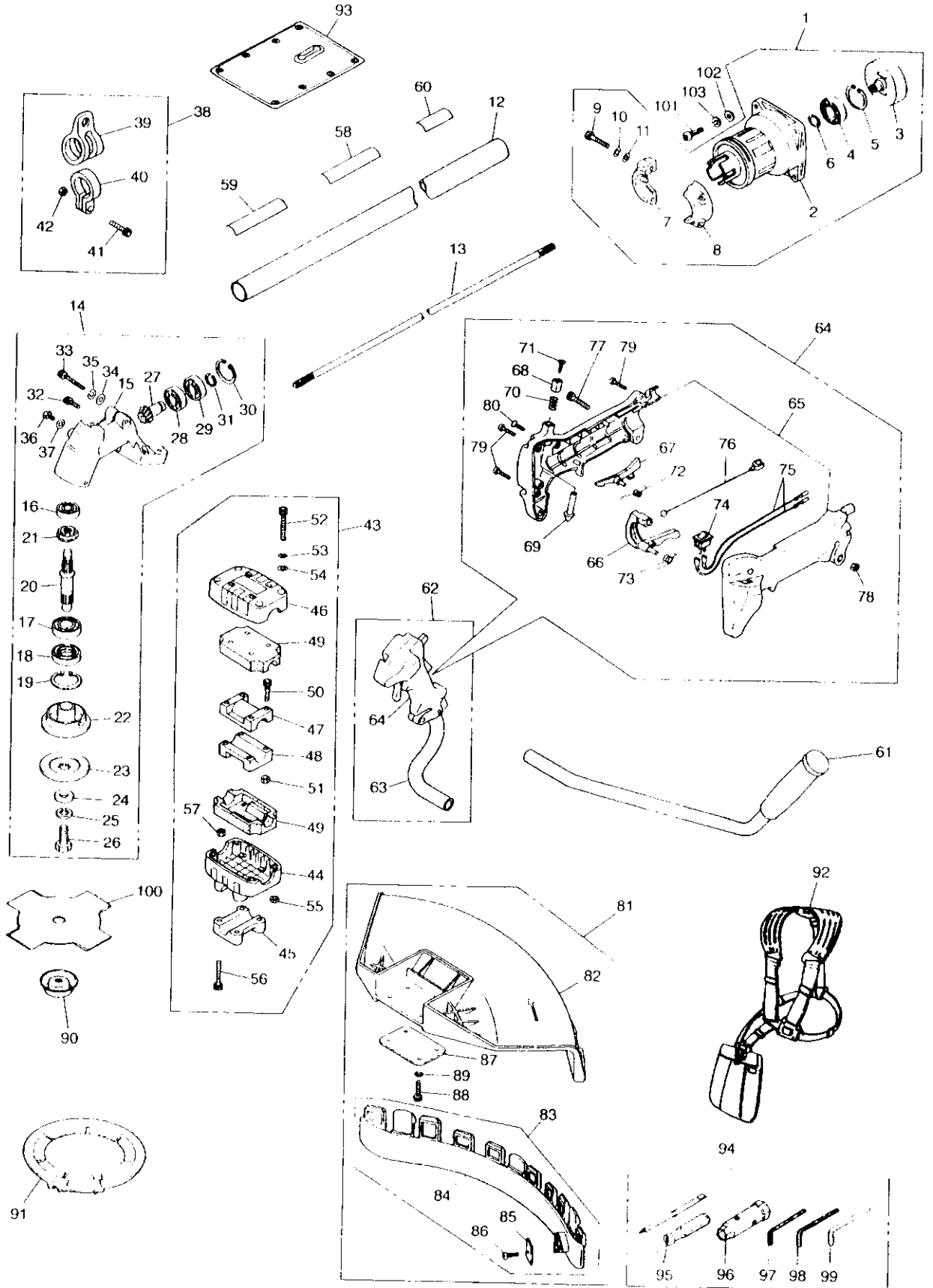
Fig.1 CUTTER GROUP
