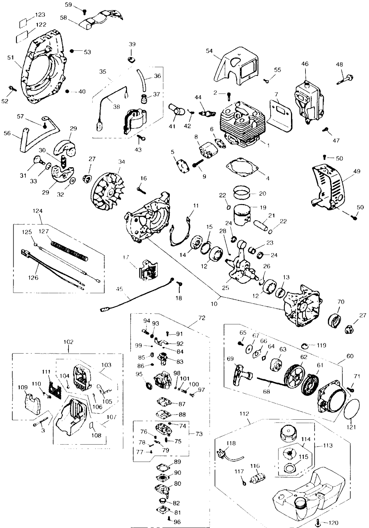
Fig.2 ENGINE GROUP
