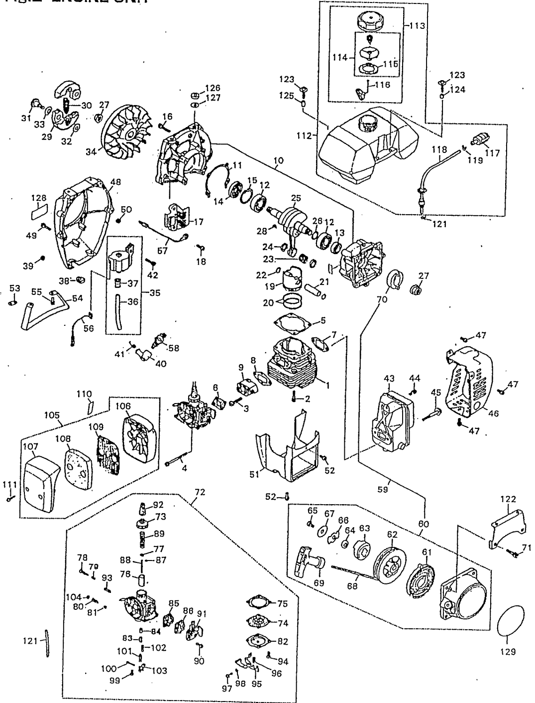
Fig.2 ENGINE UNIT
