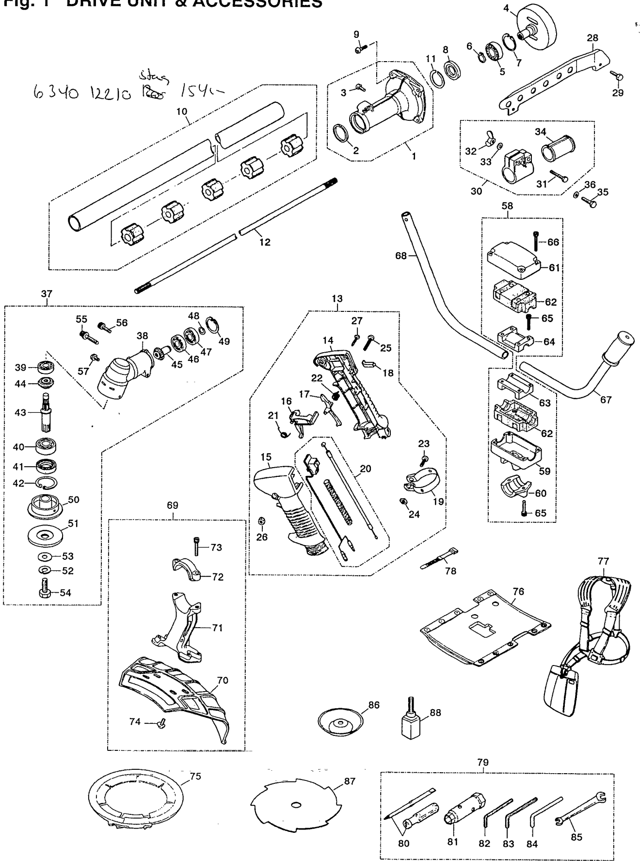
Fig. 1 DRIVE UNIT & ACCESSORIES
