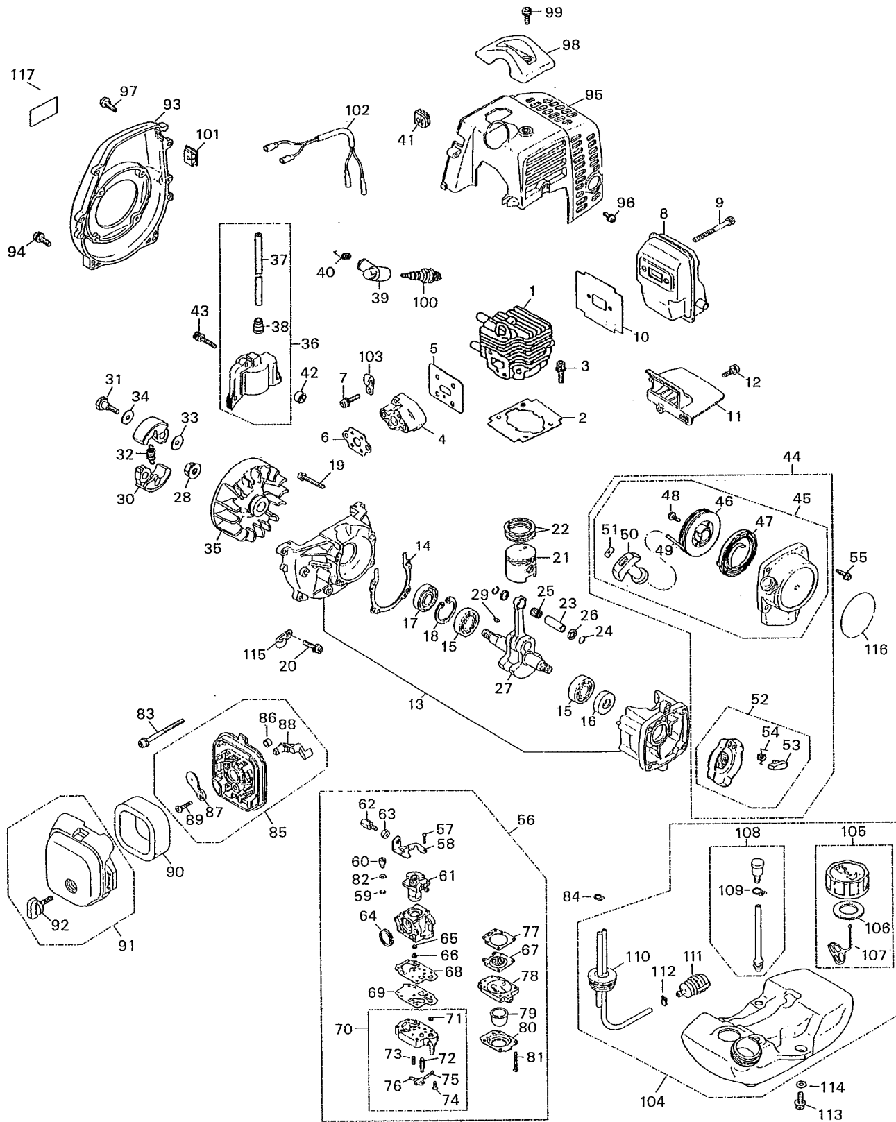
Fig.2 ENGINE GROUP
