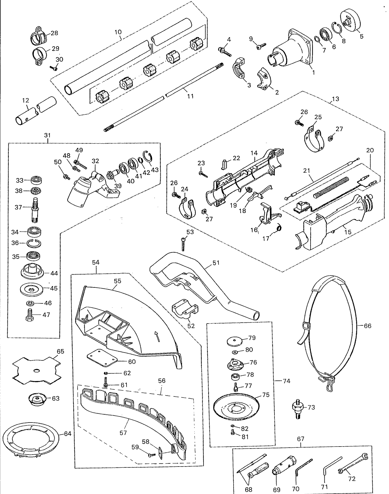
Fig.1 CUTTER GROUP
