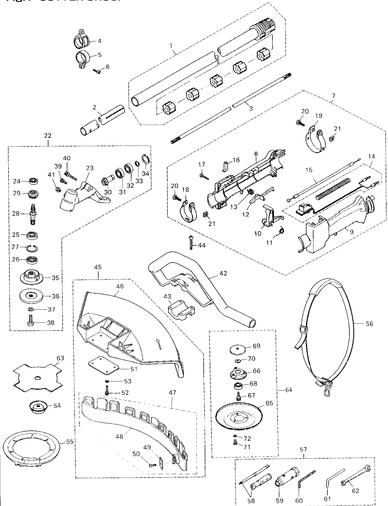
Fig.1 CUTTER GROUP
