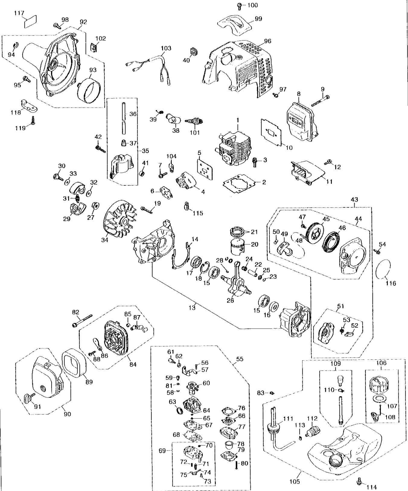
Fig.2 ENGINE GROUP
