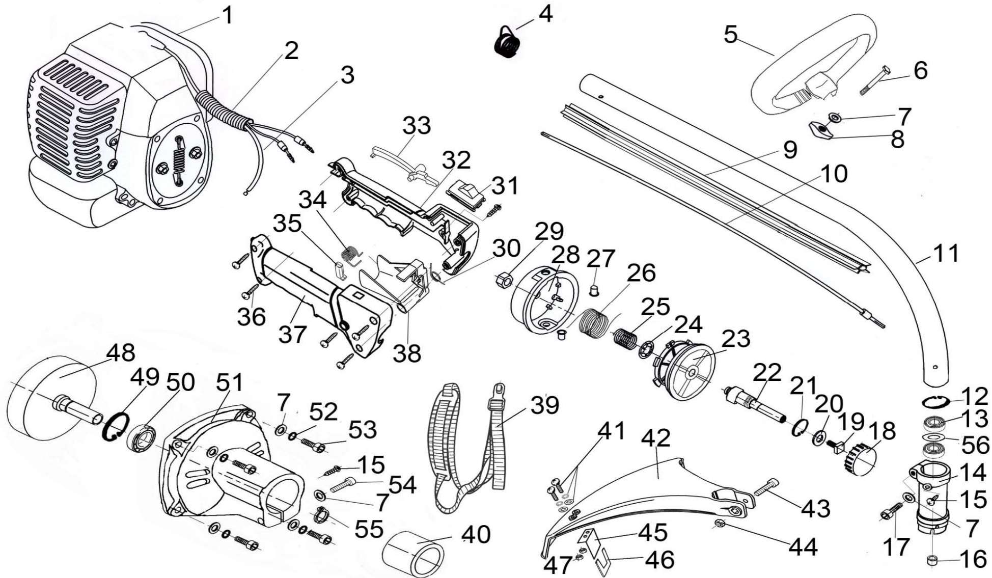
Trimmerhoved / Trimmerhaed assy 408007
